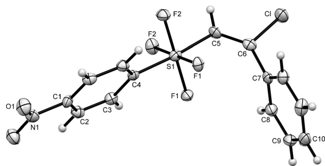
Figure 1. Molecular structure of 1c . Thermal ellipsoids are shown at 50% probability.
